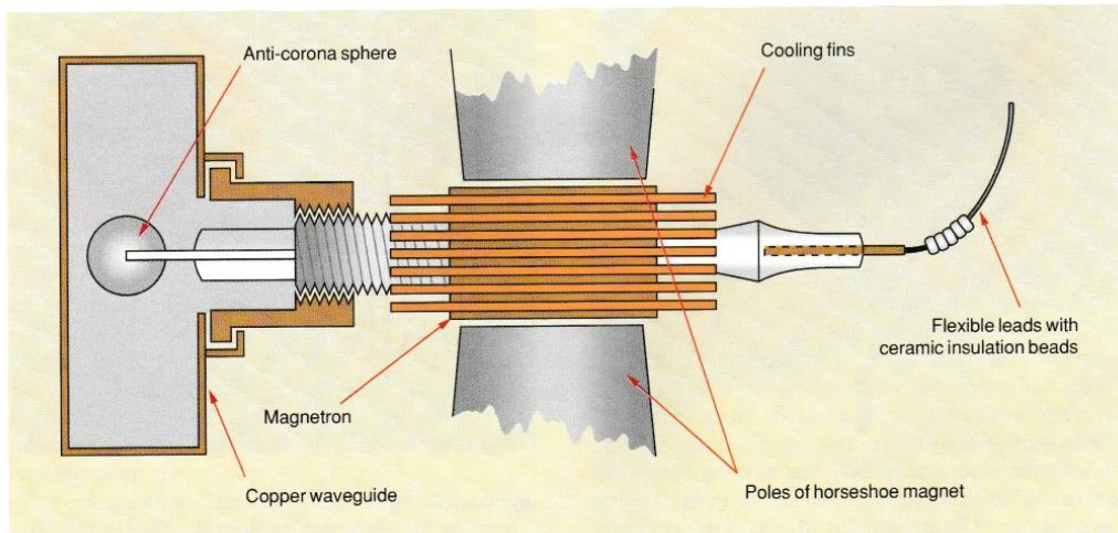
4 Detail of the magnetron/waveguide arrangement in the Type 277 radar
