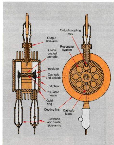
3 a) The CV76 S-band strapped magnetron, as used in the Type 277 radar. The device operated at 25 kV, 40 A and produced radiation at a wavelength of 10 cm; and b) diagrams showing construction of the magnetron
