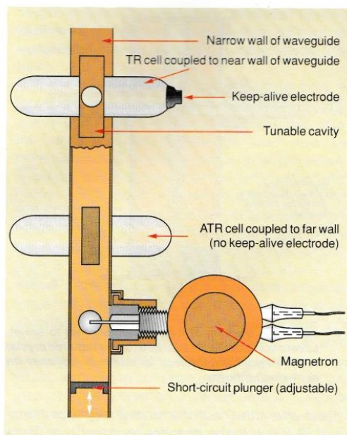
5 Diagram showing the magnetron, transmit/receive (TR) cell, ATR cell and waveguide arrangement in the Type 277 radar
